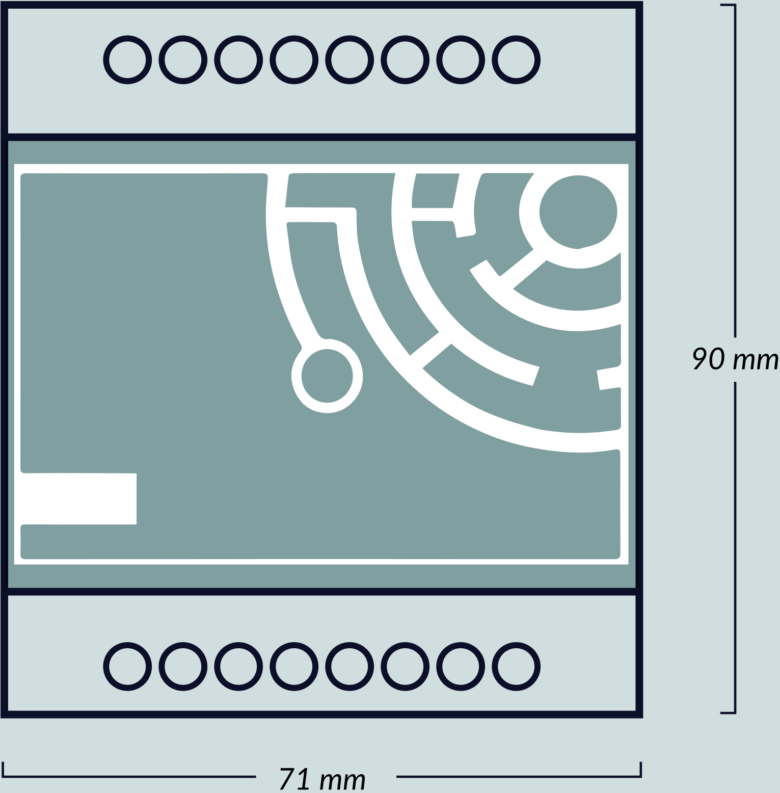
Vista frontal
